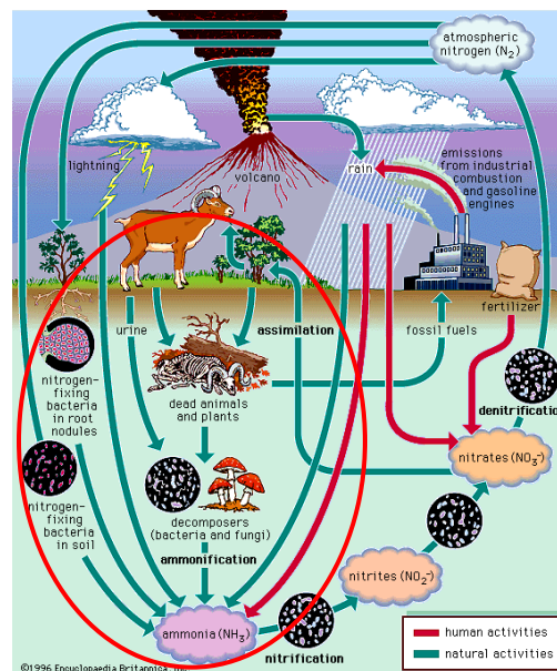
Circled area above demonstrates some of the microbial & soil forming processes associated with the normal N Cycle
